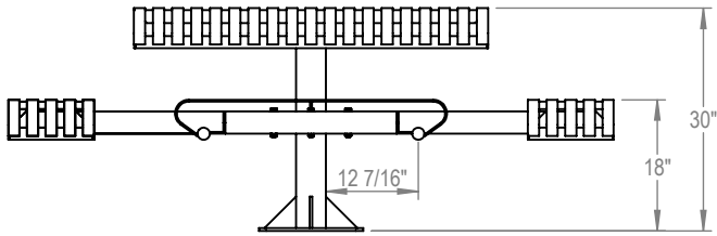
SURFACE MOUNT
